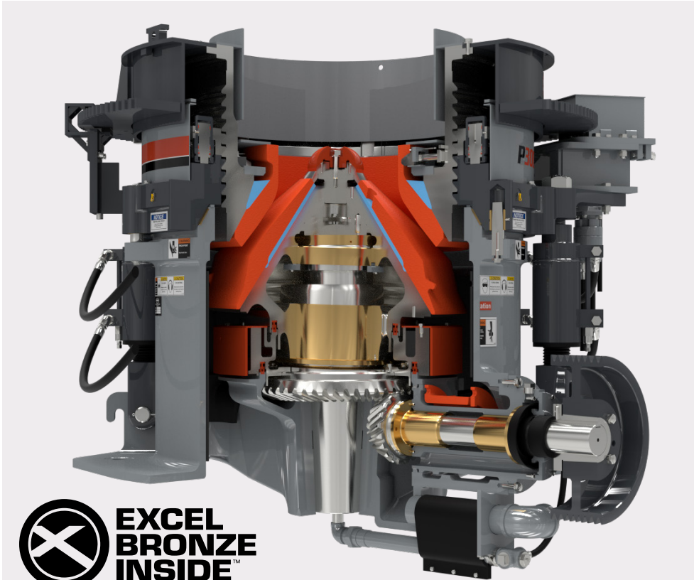
MODEL SHOWN: P300 CUT-AWAY
