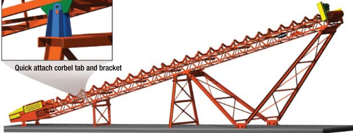
Tail Support
